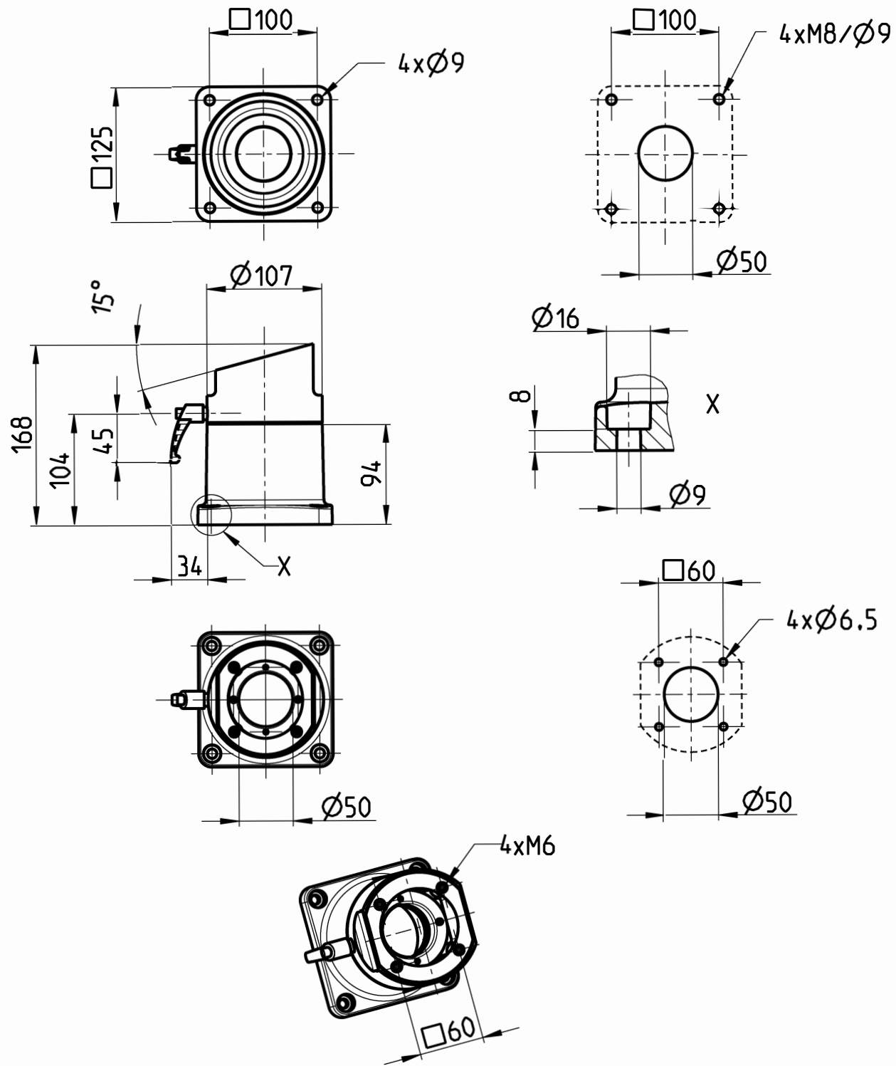
1015300184 Neig-Standf-kupplung 15°A
