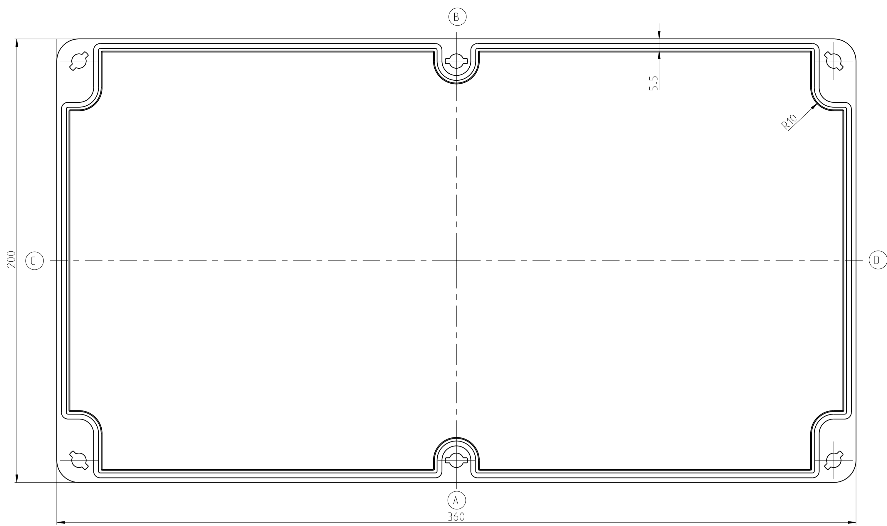
DECKEL/LID/COUVERCLE
