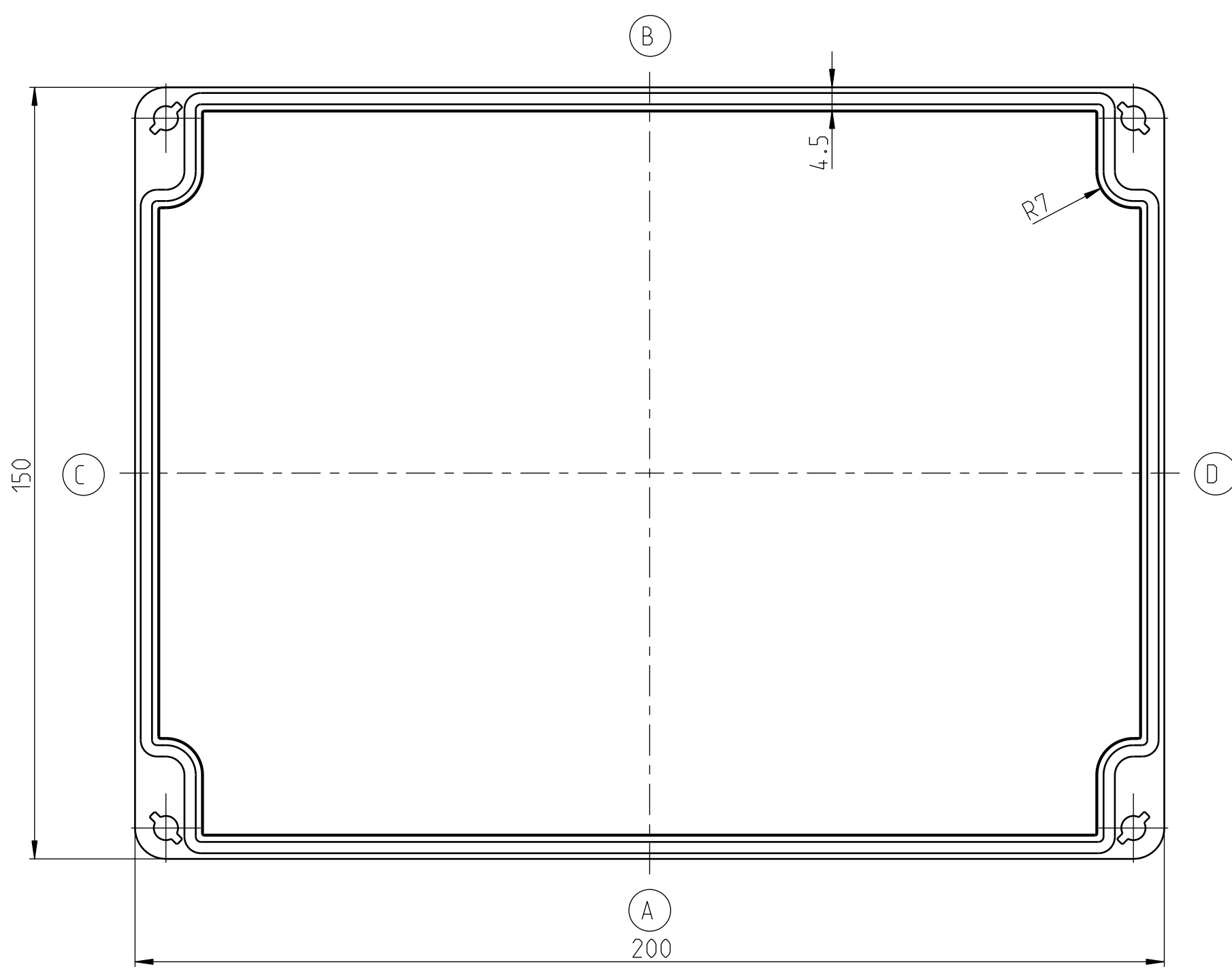
DECKEL/LID/COUVERCLE
