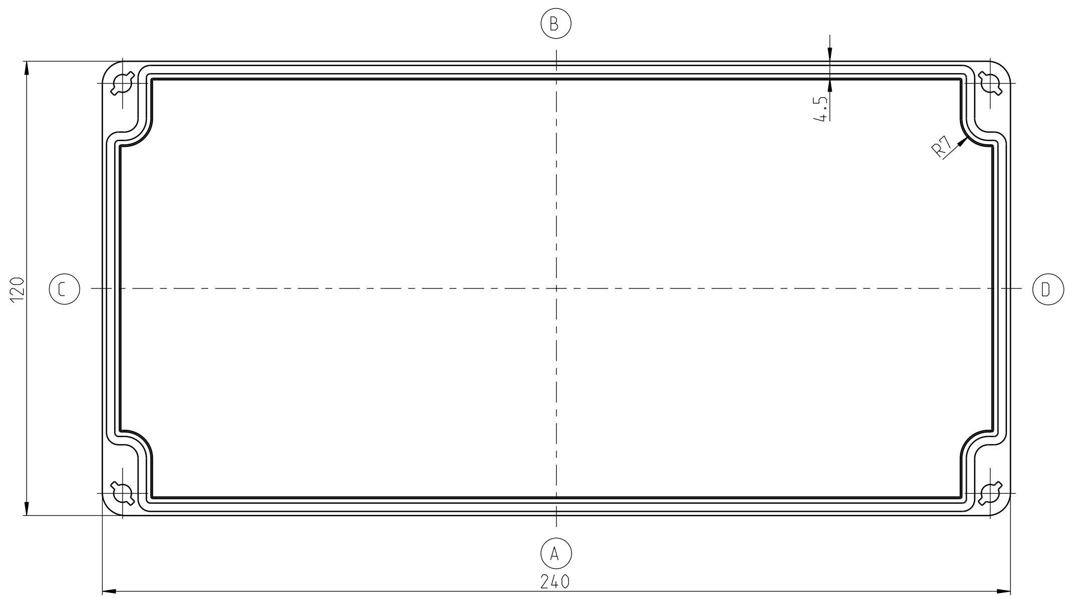
DECKEL/LID/COUVERCLE
