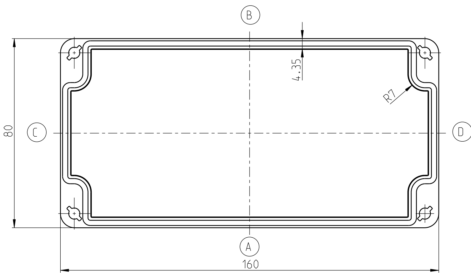
DECKEL/LID/COUVERCLE
