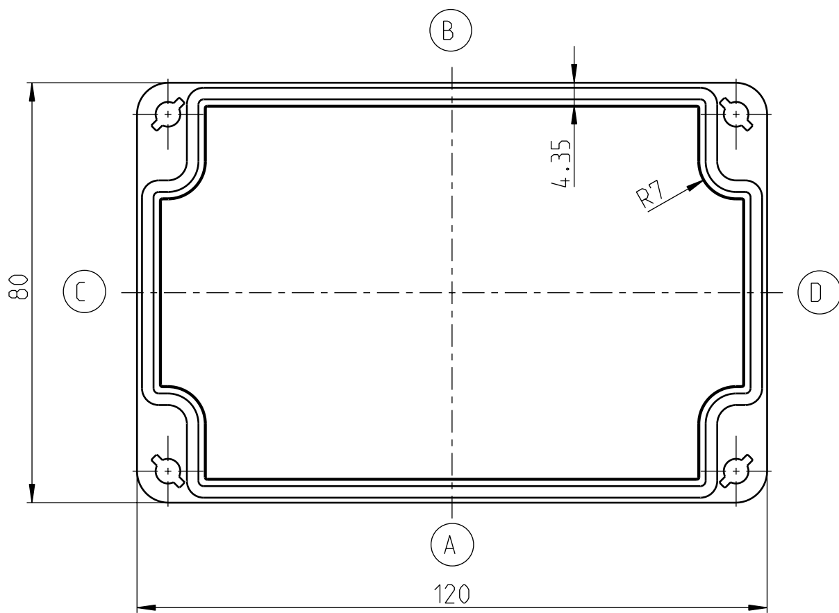
DECKEL/LID/COUVERCLE
