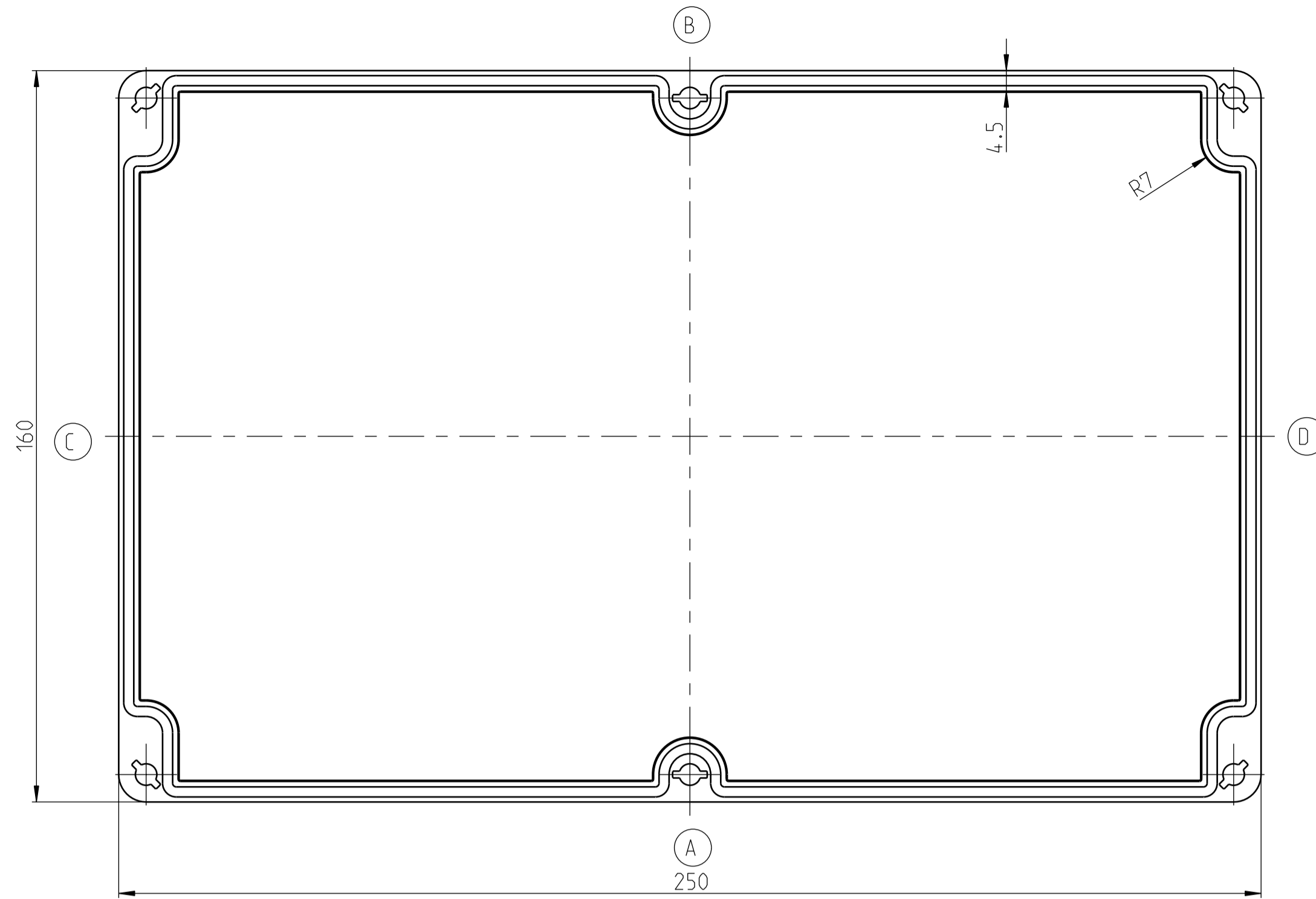
DECKEL/LID/COUVERCLE
