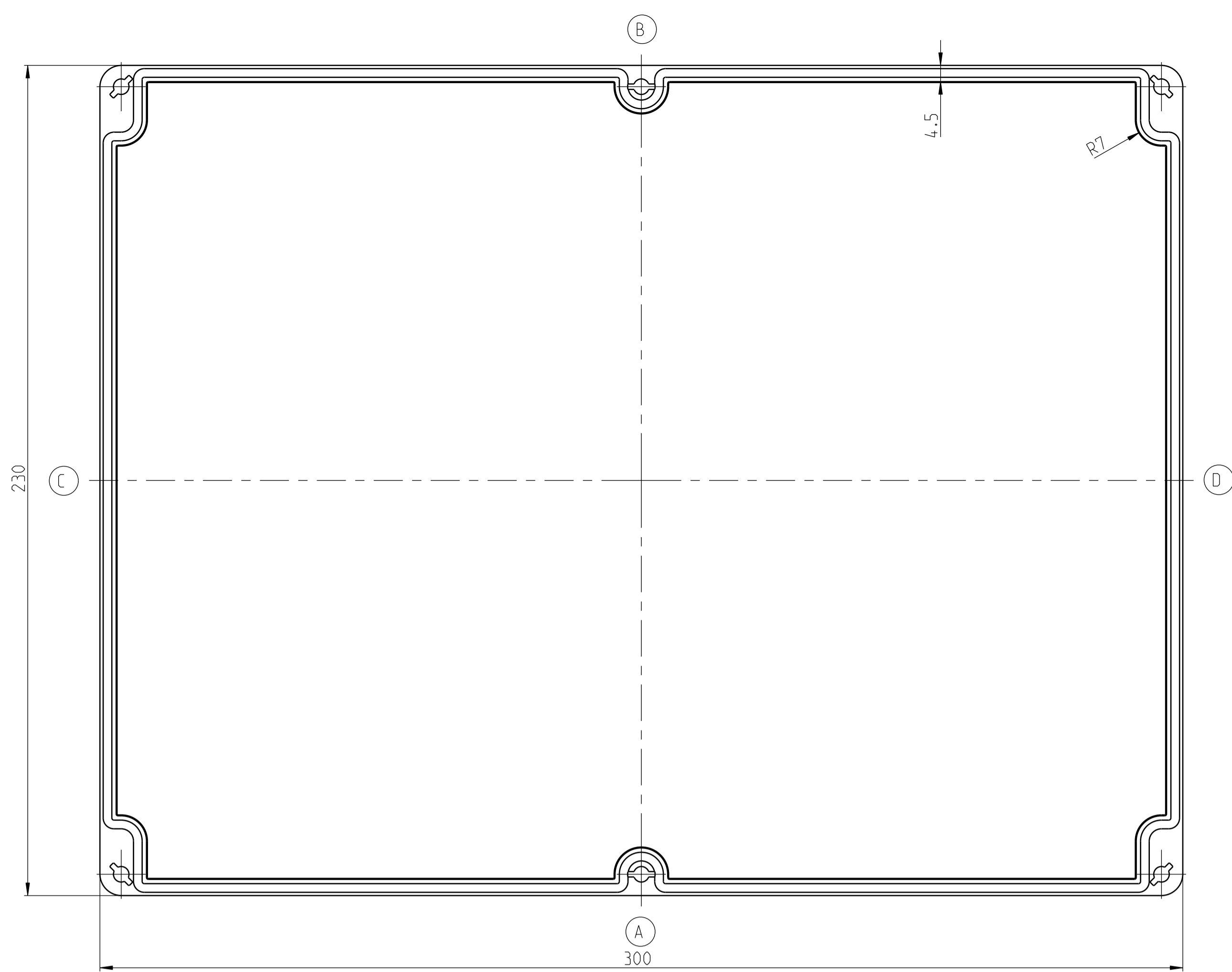
DECKEL/LID/COUVERCLE
