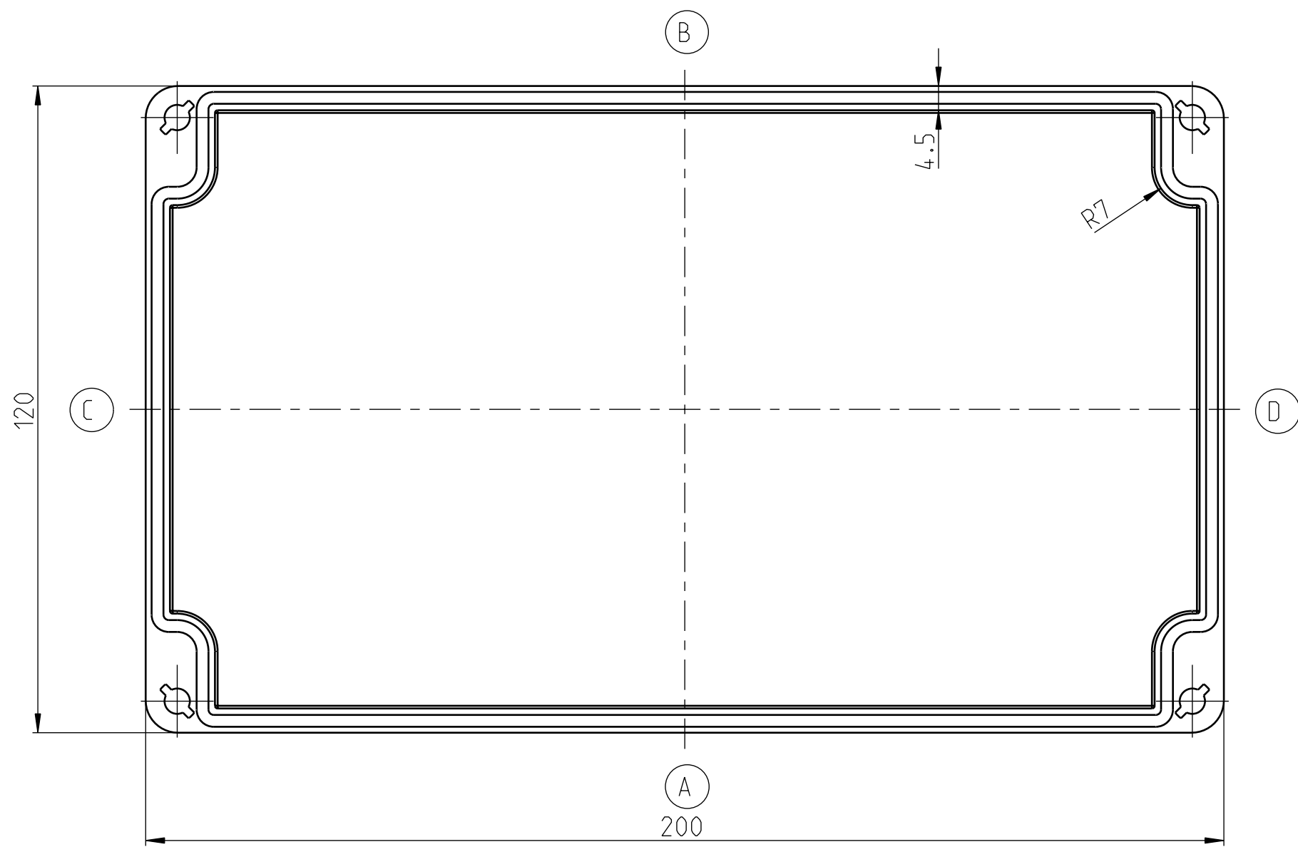
DECKEL/LID/COUVERCLE
