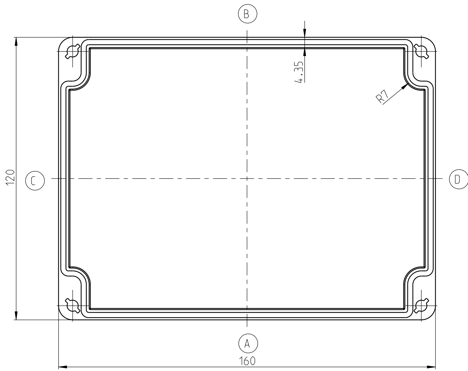
DECKEL/LID/COUVERCLE
