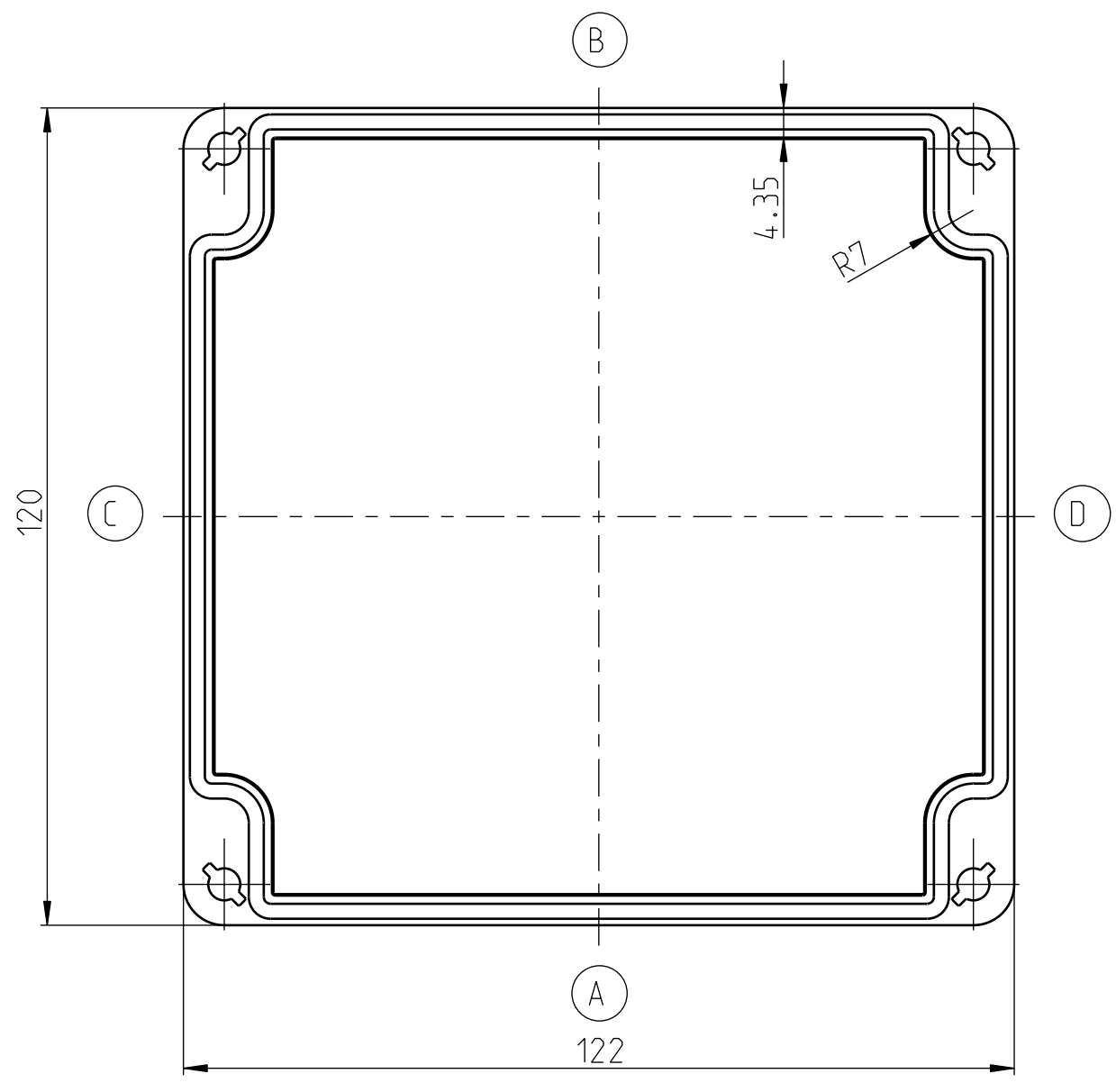
DECKEL/LID/COUVERCLE
