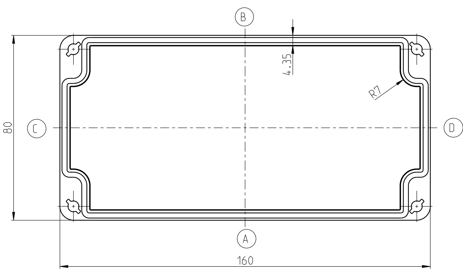
DECKEL/LID/COUVERCLE
