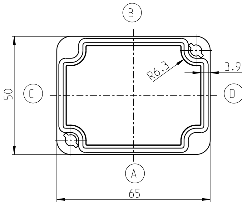
DECKEL/LID/COUVERCLE
