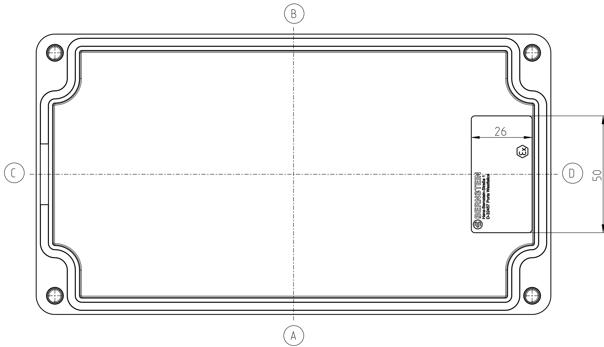
DECKEL
