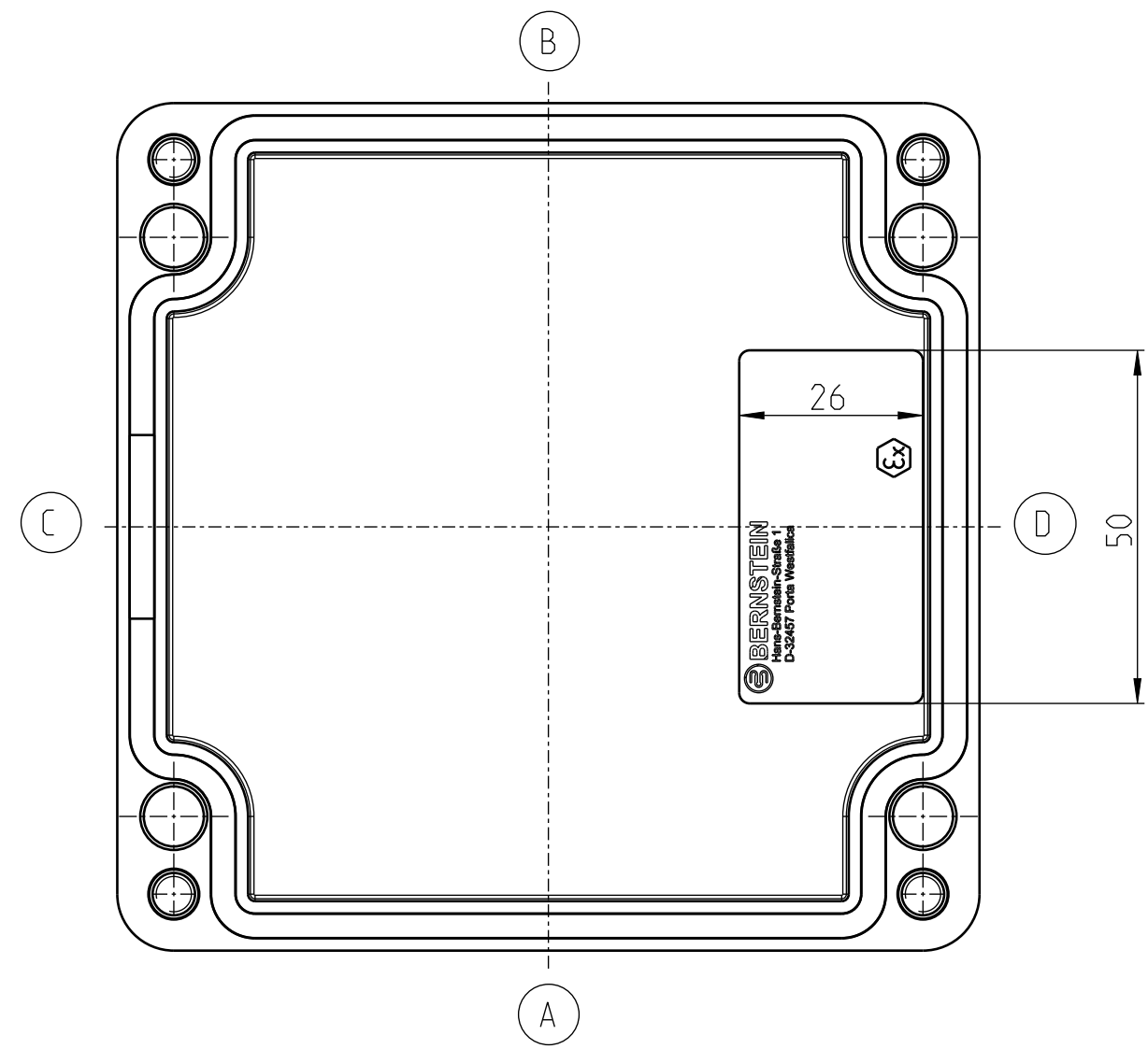
DECKEL
