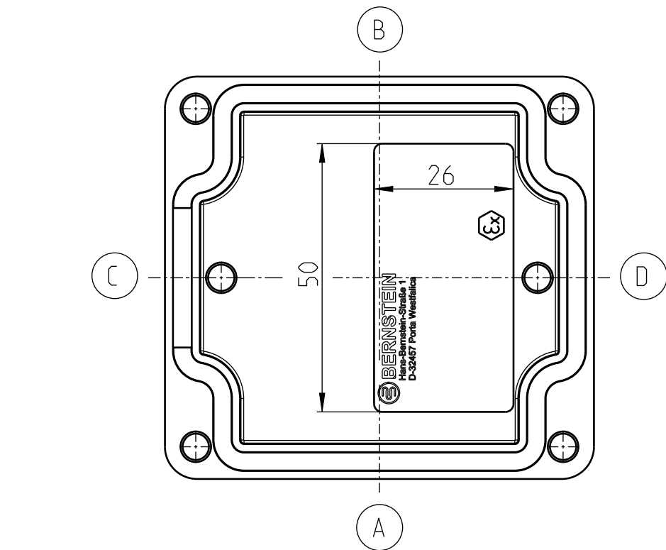
DECKEL
