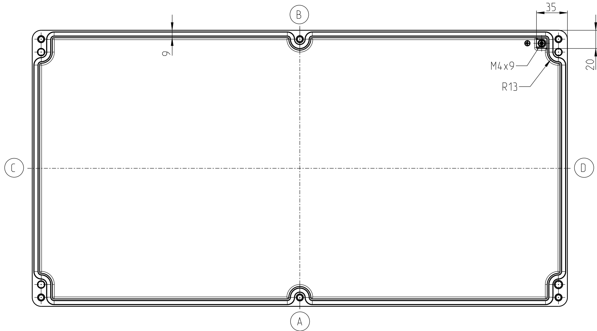
DECKEL
