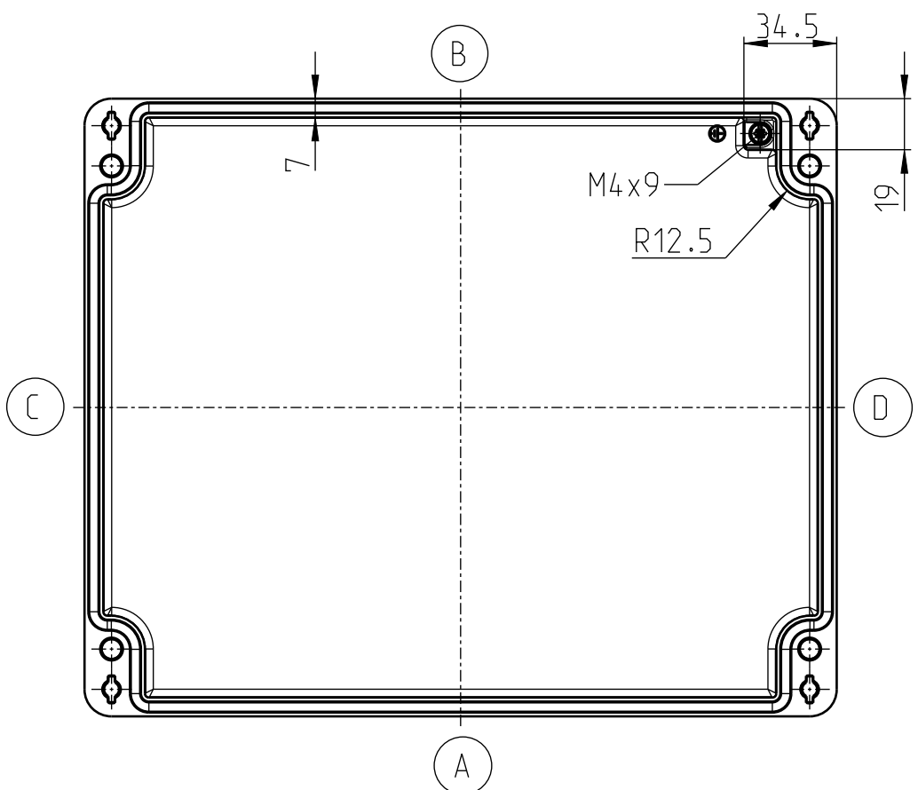
DECKEL
