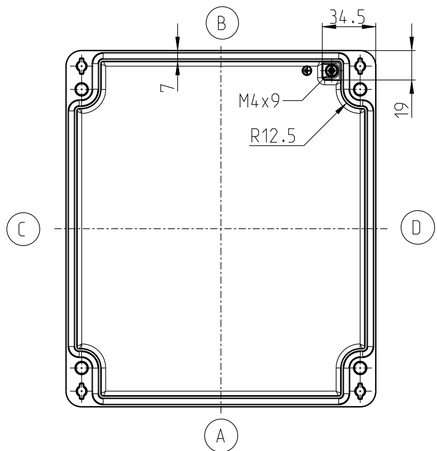
DECKEL
