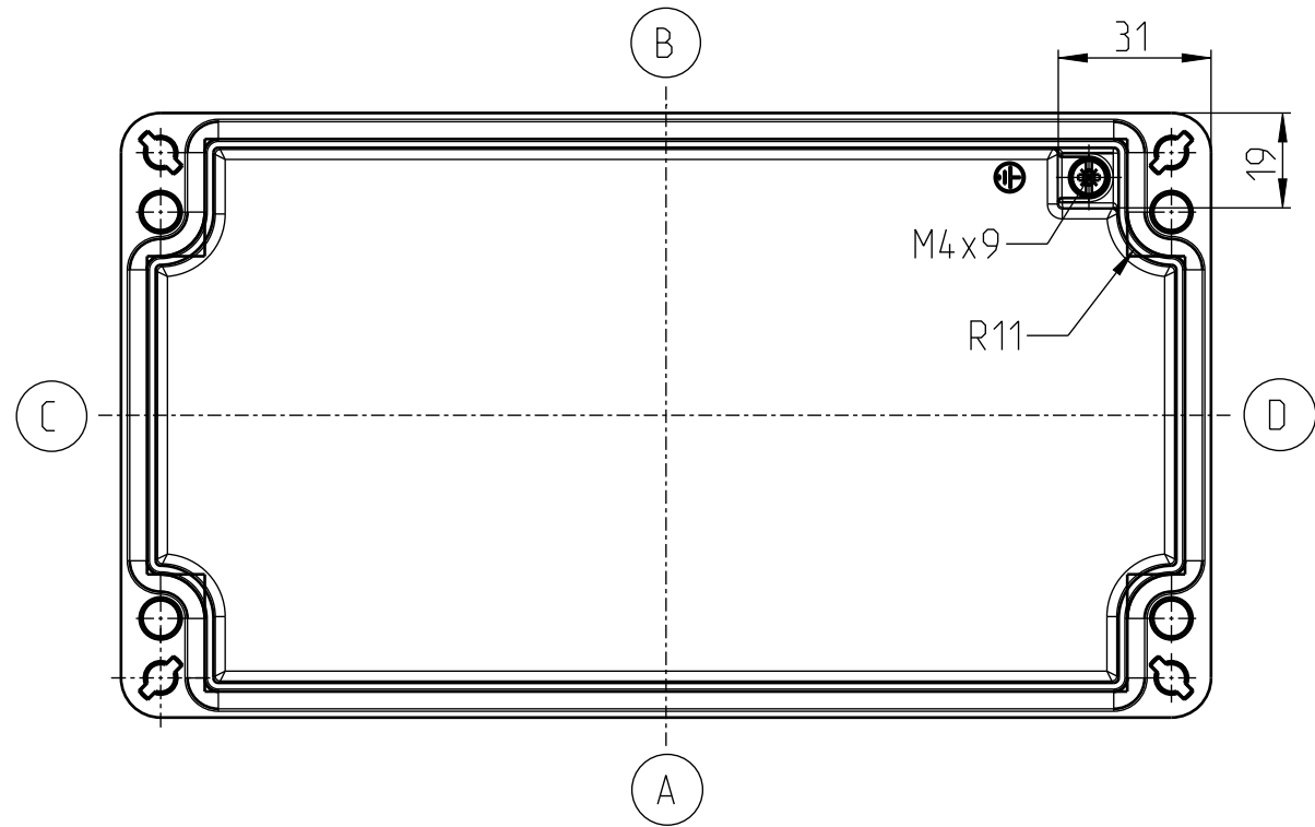
DECKEL
