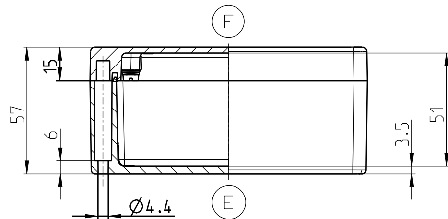
DECKEL
