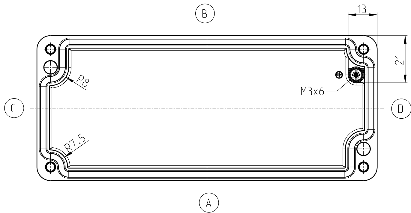
DECKEL
